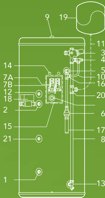
Schematic for 250 & 300 litre only
